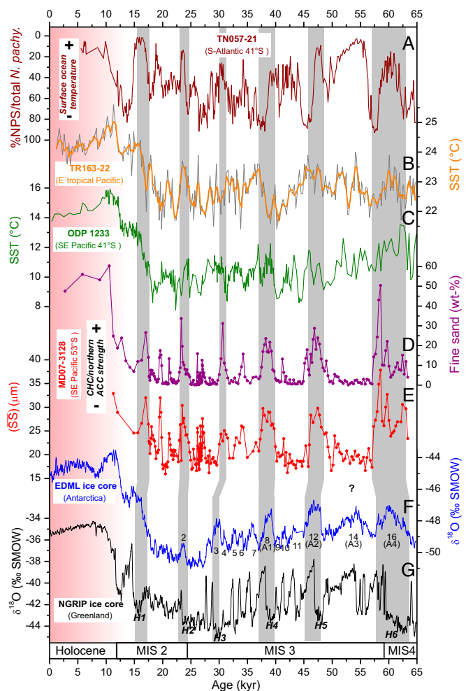
Fig. 4. Reconstructed changes in CHC strength and DP throughflow compared with temperature records. (A) Ratio of planktonic foraminifera Neogloboquadrina pachyderma (NPS) to total NPS counts indicative of surface ocean temperature changes in the South Atlantic (42). (B) Mg/Ca SST record from the Galapagos region (43) representing eastern tropical Pacific SST changes. (C) Alkenone SST record from Ocean Drilling Program (ODP) Site 1233 located within the Humboldt Current System (HCS) at ~41° S (20) (updated age model) ( SI Methods ). (D and E) Fine-sand (63–150 μm) contents and \overline{SS} as proxies for CHC/northern ACC strength. (F) Oxygen isotope record of the east Antarctic European Project for Ice Coring in Antarctica Dronning Maud Land Ice Core (EDML) ice core (36) [Antarctic ice core chronology (AICC) 2012 age scale]. Numbers mark Antarctic Isotope Maxima and the largest Antarctic warmings from A1 to A4. (G) Oxygen isotope record of the Greenland North Greenland Ice Core Project ice core (36) (Greenland Ice Core Chronology 2005 age scale). Vertical gray bars mark inferred millennial-scale DP throughflow peaks that correspond with millennial-scale temperature maxima in Antarctica and Heinrich stadials (Hs) in Greenland. MIS, marine isotope stages; SMOW, standard mean ocean water.
